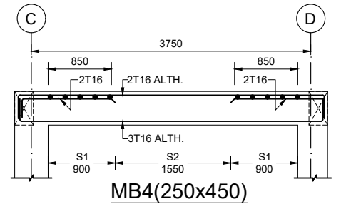
MUMMTY BEAM REINFORCEMENT DETAILS
