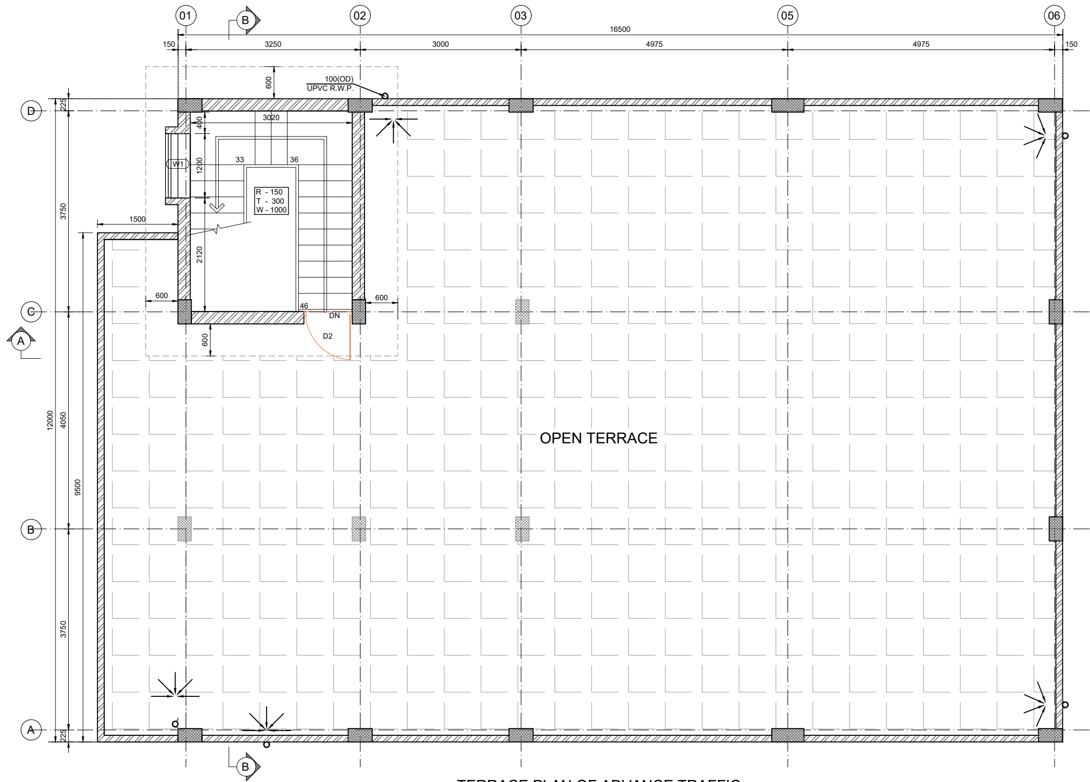
TERRACE PLAN OF ADVANCE TRAFFIC MANAGEMENT SYSTEM (ATMS) BUILDING
