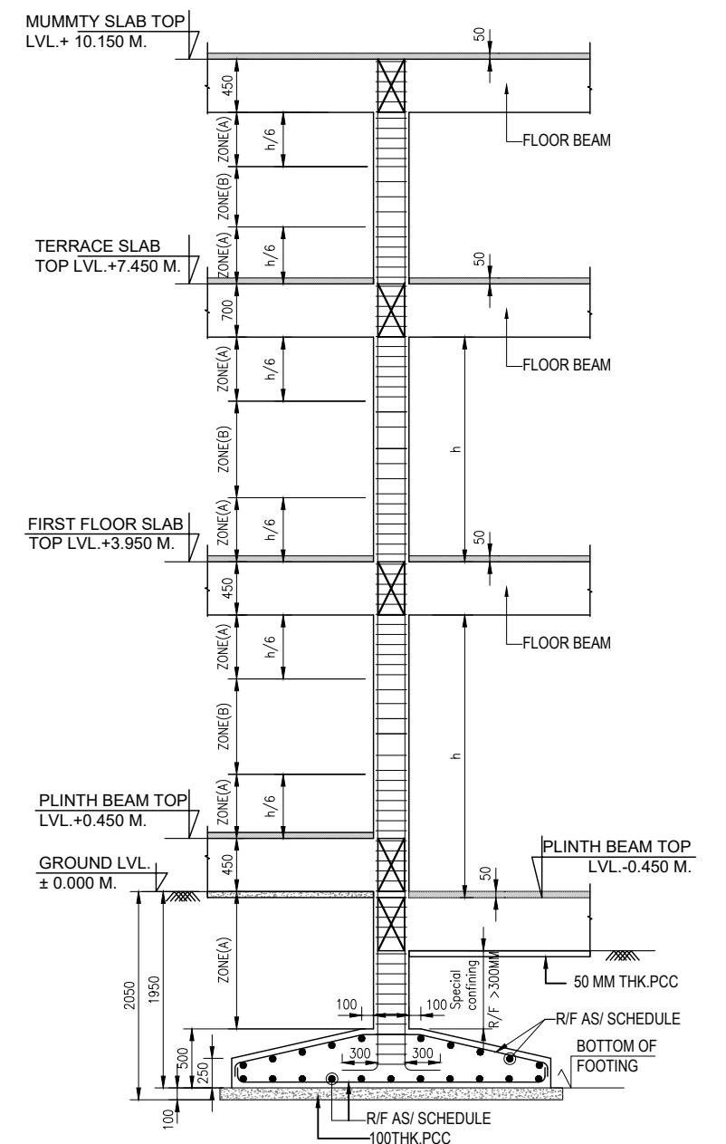
TYPICAL DETAIL OF COLUMN - C1 & C2 SCALE - 1:40
