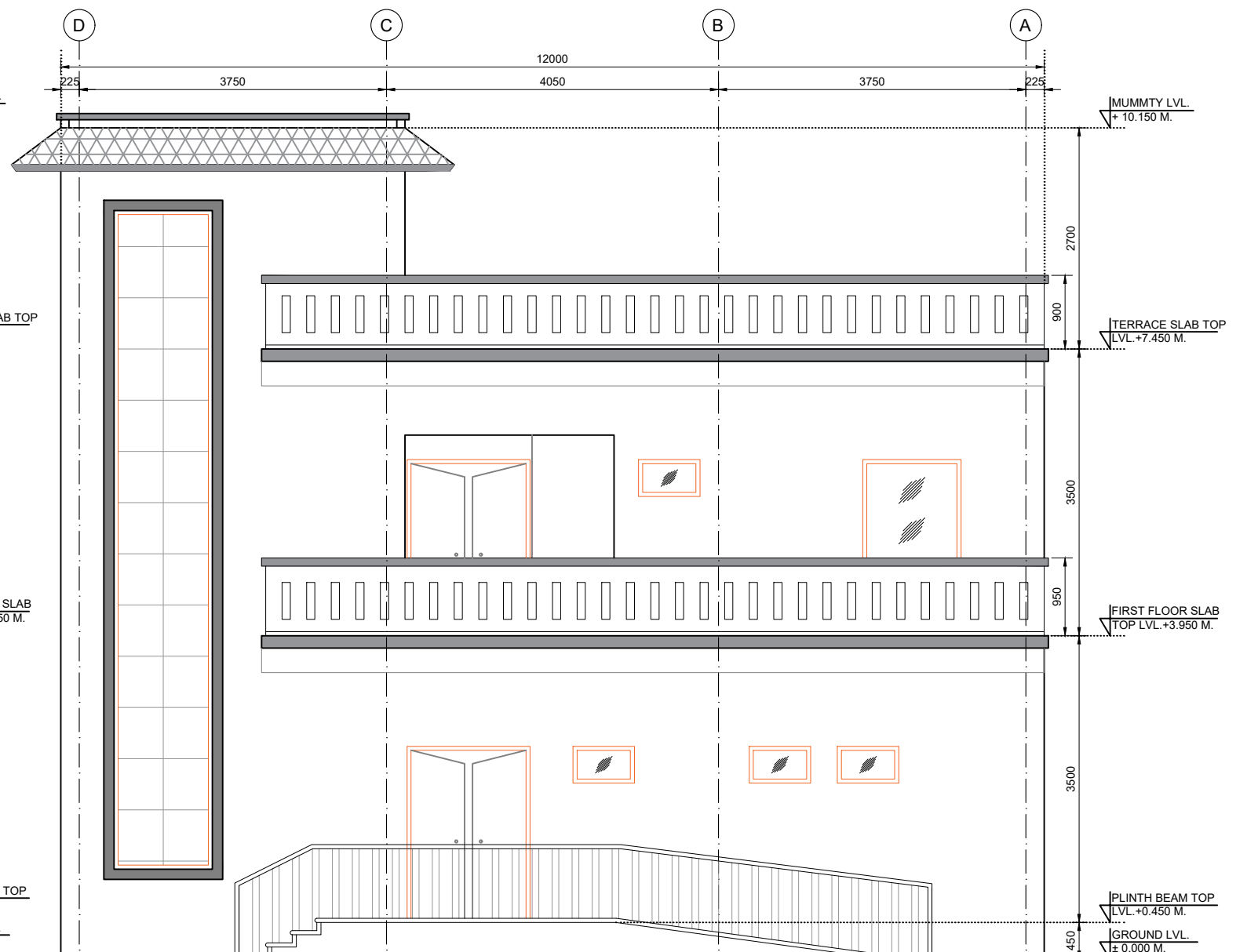
FRONT ELEVATION
