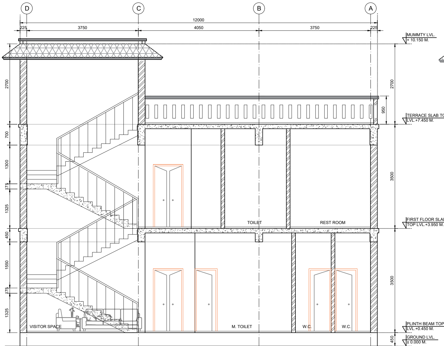
SECTION B-B
