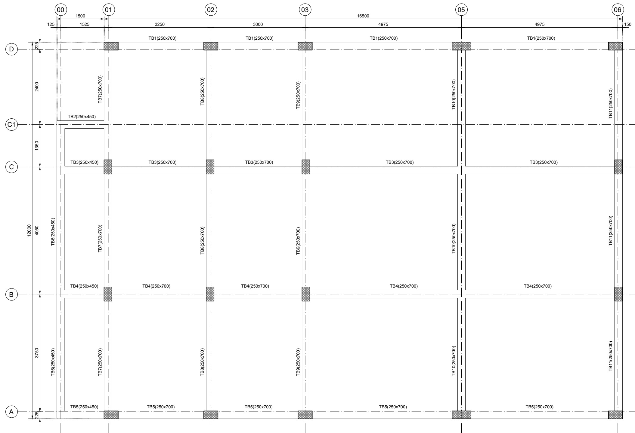
TERRACE SLAB BEAM LAYOUT PLAN
