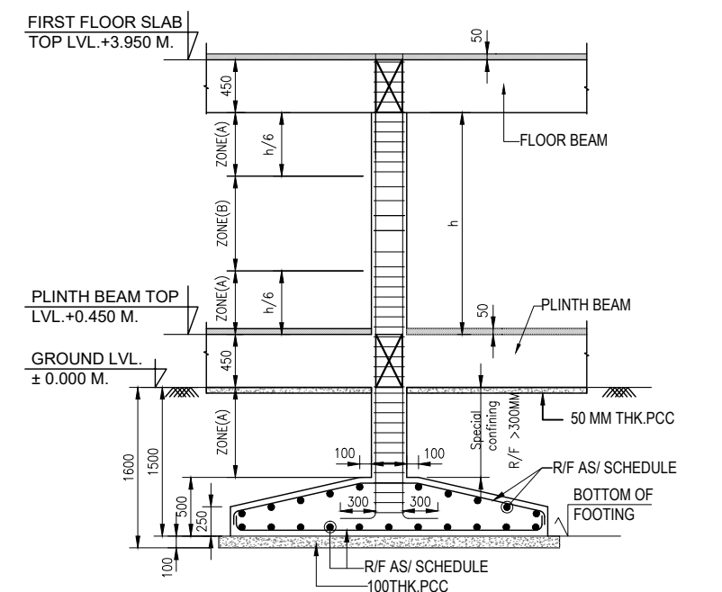
TYPICAL DETAIL OF COLUMN - C3 SCALE - 1:40
