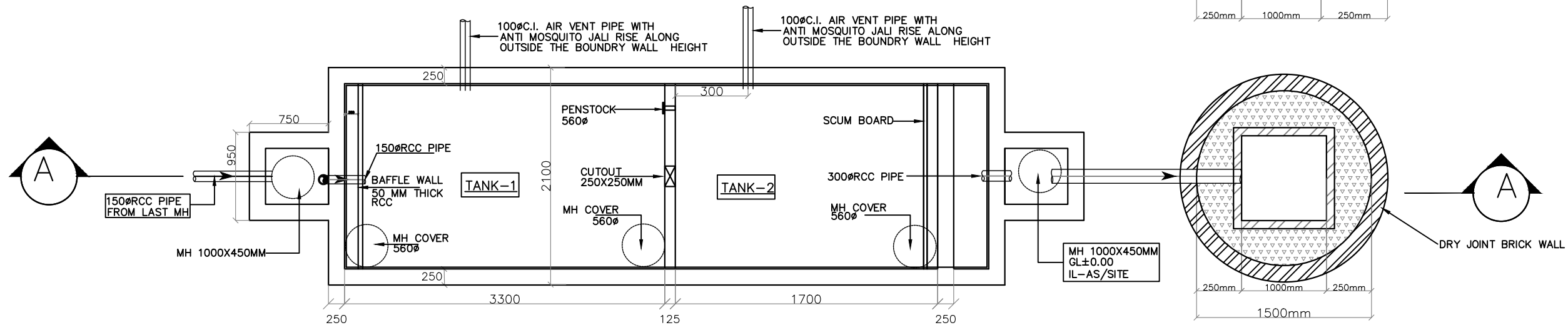
PLAN SEPTIC TANK
