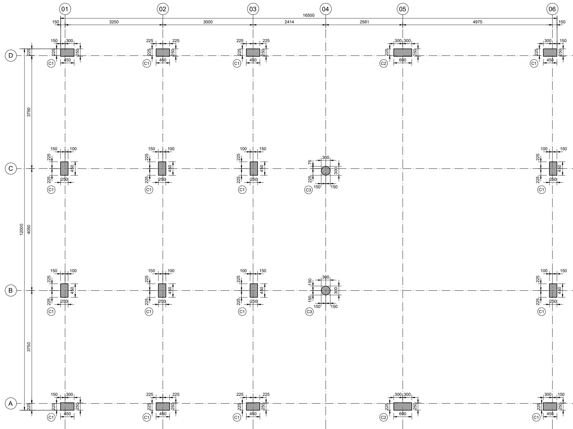
COLUMN LAYOUT PLAN OF ADVANCE TRAFFIC MANAGEMENT SYSTEM (ATMS) BUILDING
