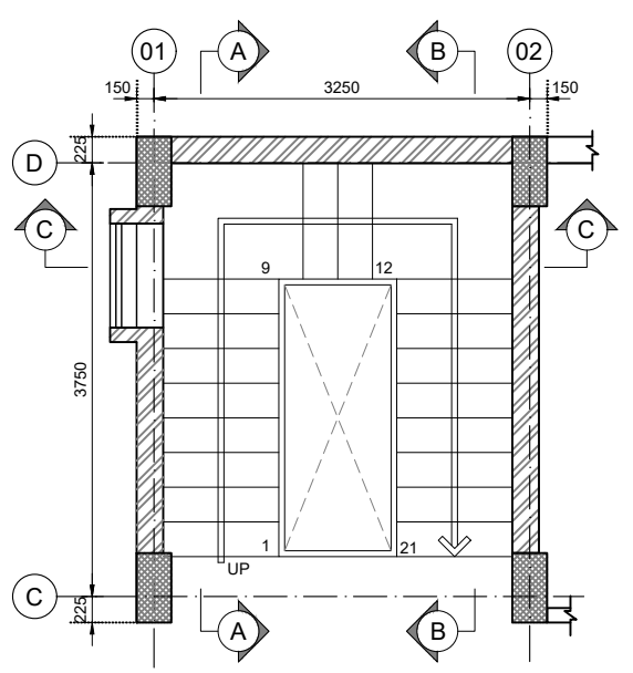
STAIRCASE
