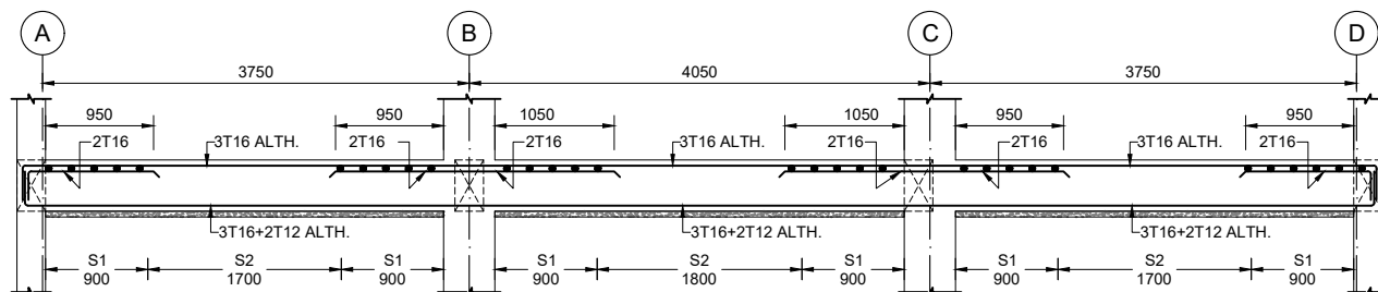
GB8(250x450)
