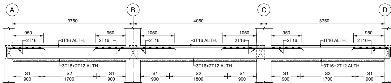
GB10(250x450)
