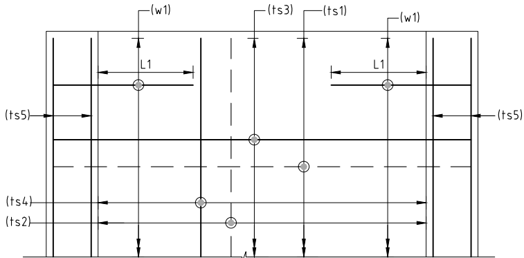
TOP SLAB REINFORCEMENT
